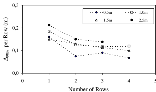
Figure 8. Frontal displacement at 90% of the maximum pullout load per number of rows, for different surcharge heights.
