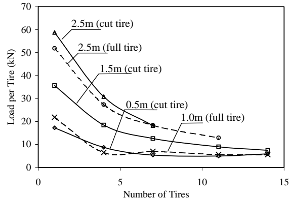
Figure 3. Maximum load normalized behavior.
